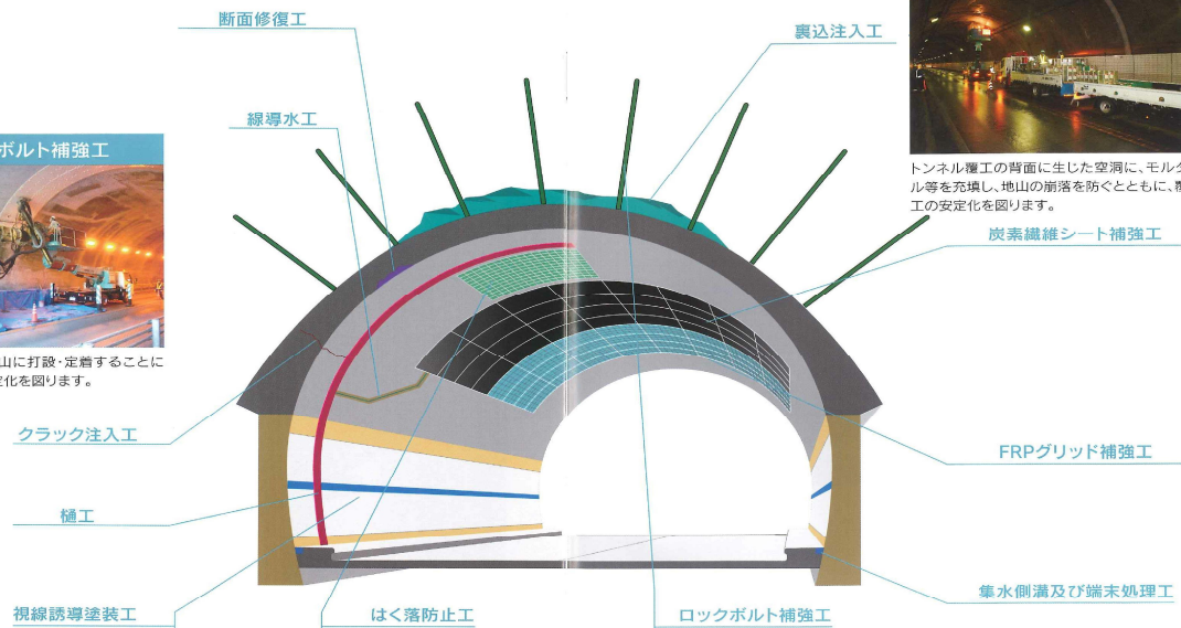
裏込注入工
